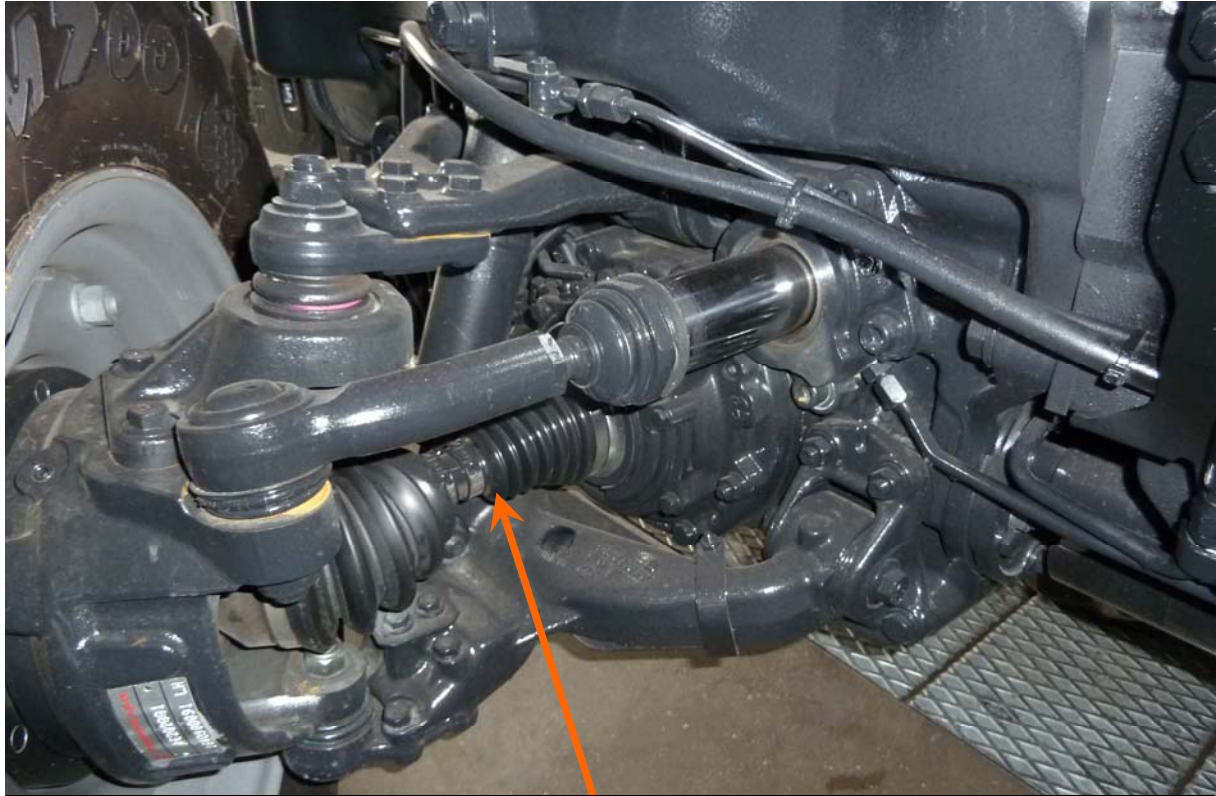
ASSALE CON PONTE SOSPESO AXLE WITH SUSPENSION BRIDGE
